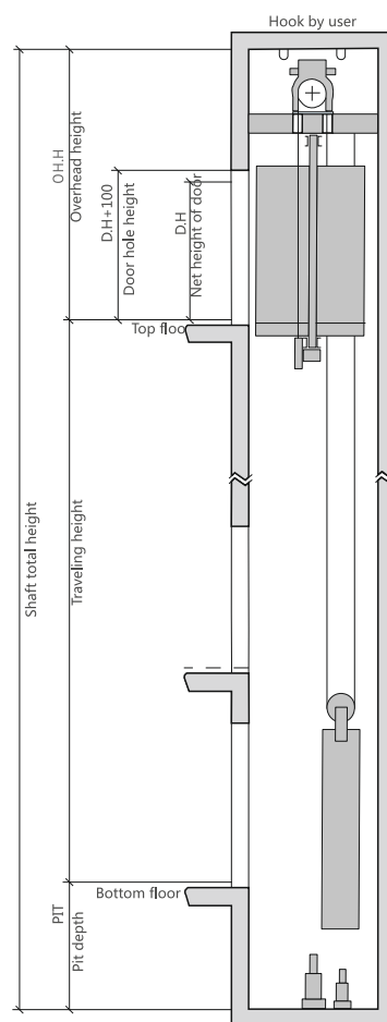
Hoistway vertical layout
