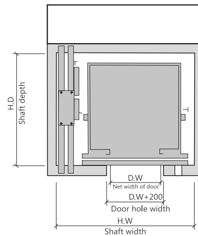
Top floor plan layout
